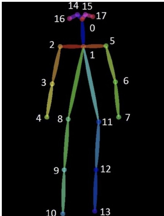
POSE ESTIMATION
